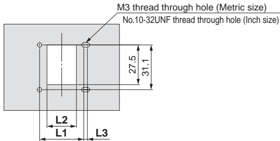
Panel fitting dimensions/Mounting hole dimensions
