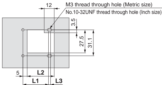
Panel fitting dimensions/Mounting hole dimensions
