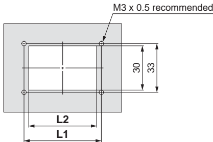
Panel fitting dimensions/Mounting hole dimensions
