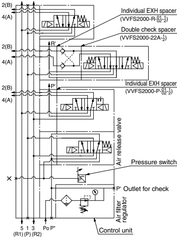
Example for manifold
