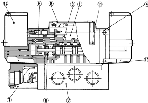
3 position closed center/exhaust center/pressure center
