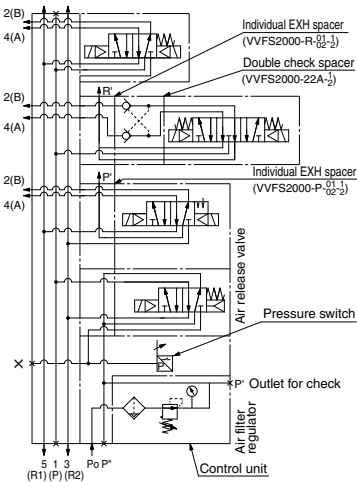
Example for manifold
