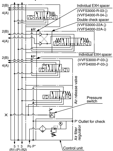
Example for manifold
