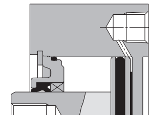
B-B section (Port on head end)
