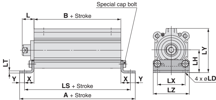
Compact Foot
