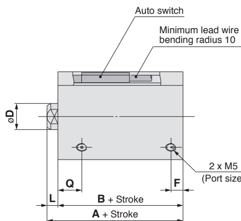
With boss on head side
