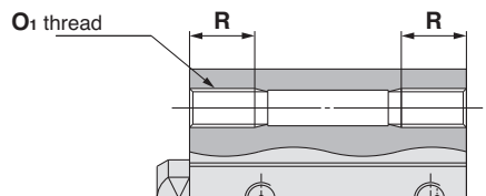
Both ends tapped: CQ2A
