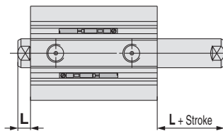
Rod end female thread
