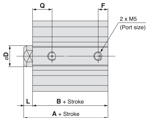
With boss on head side
