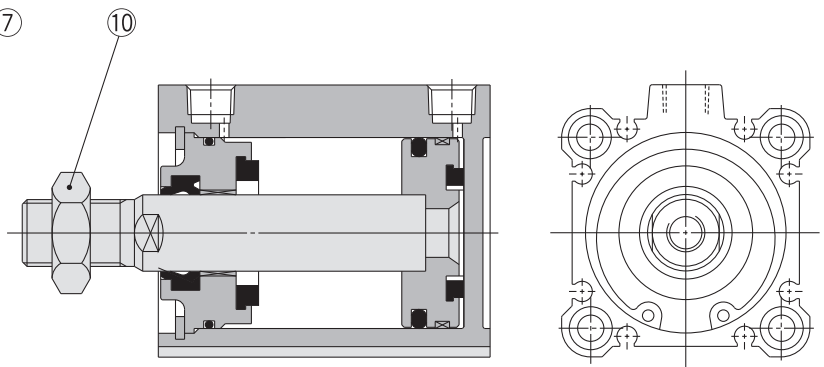
Rod end male thread
