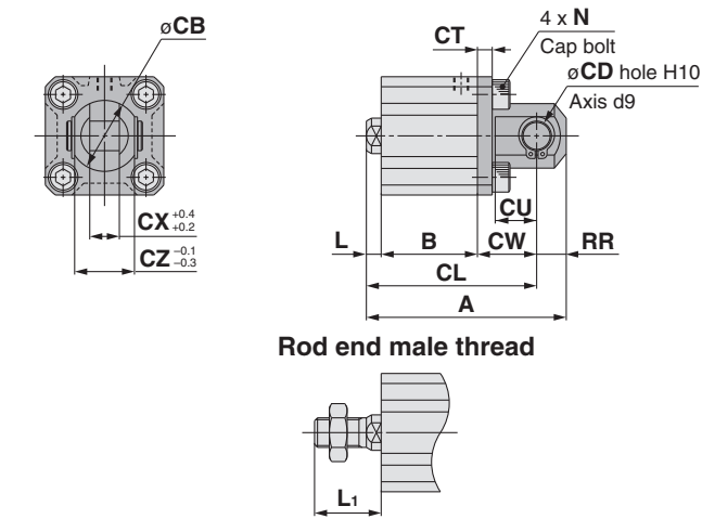
Double Clevis (mm)
