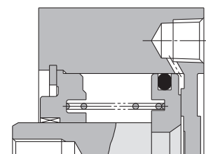
B-B section (Port on head side)
