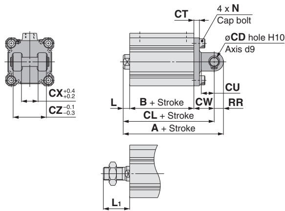
Double Clevis (mm)
