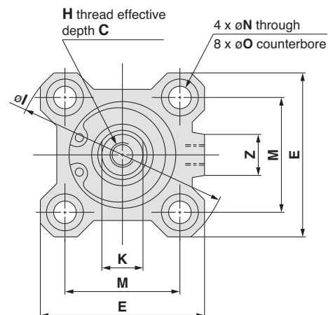
With Boss on Head side
