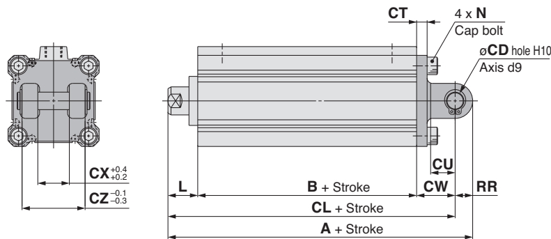
Double Clevis (mm)
