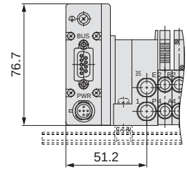
[Communication connector D-sub]
