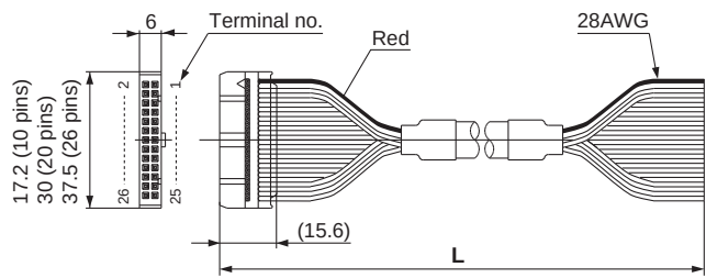
Flat ribbon cable connector
